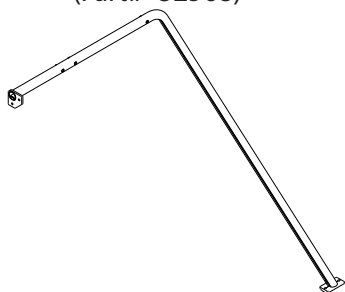
Left Backstay (1) (Part# UZ968)
