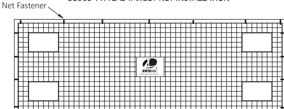
3B903 TYPICAL TARGET NET INSTALLATION
